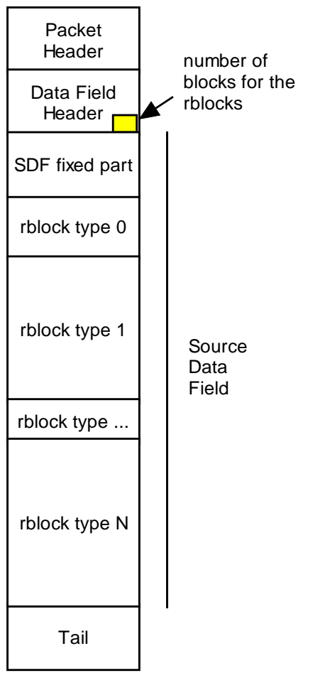
Figure 5.5: packet with rblocks
