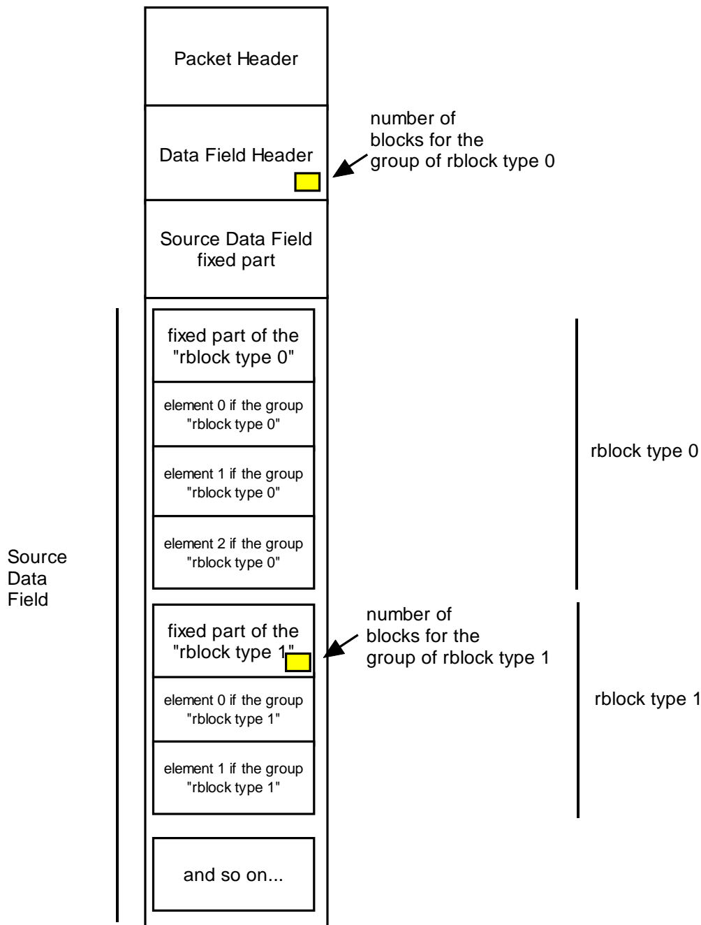
Figure 5.7: telemetry instance point of view
