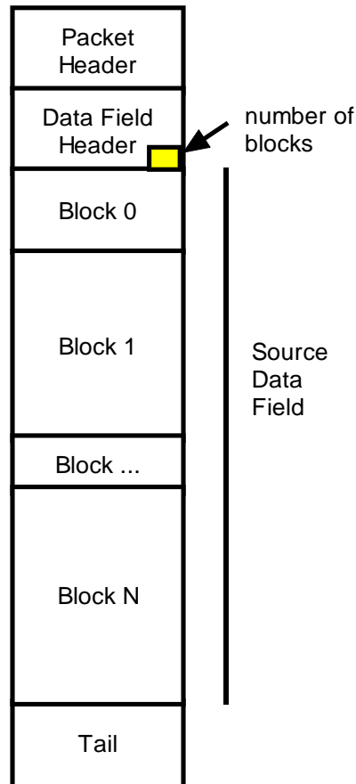
Figure 5.3: Layout 3 Packet structure
